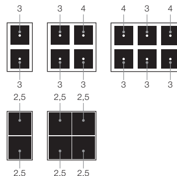
Electric plates power (kW)
